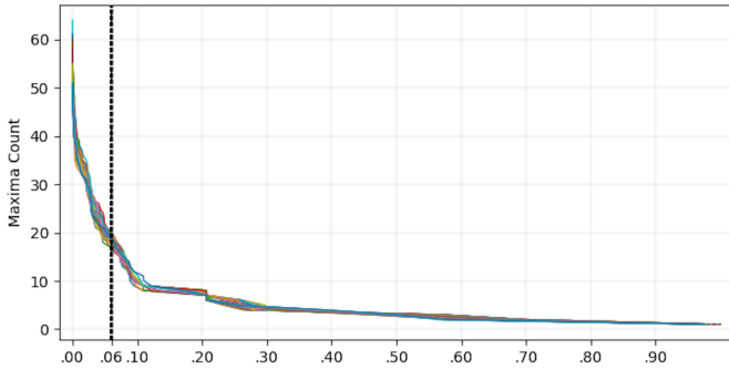
Fig. 4. Heated Cylinder: persistent simplification \varepsilon = 6\% ; x-axis is \varepsilon .
